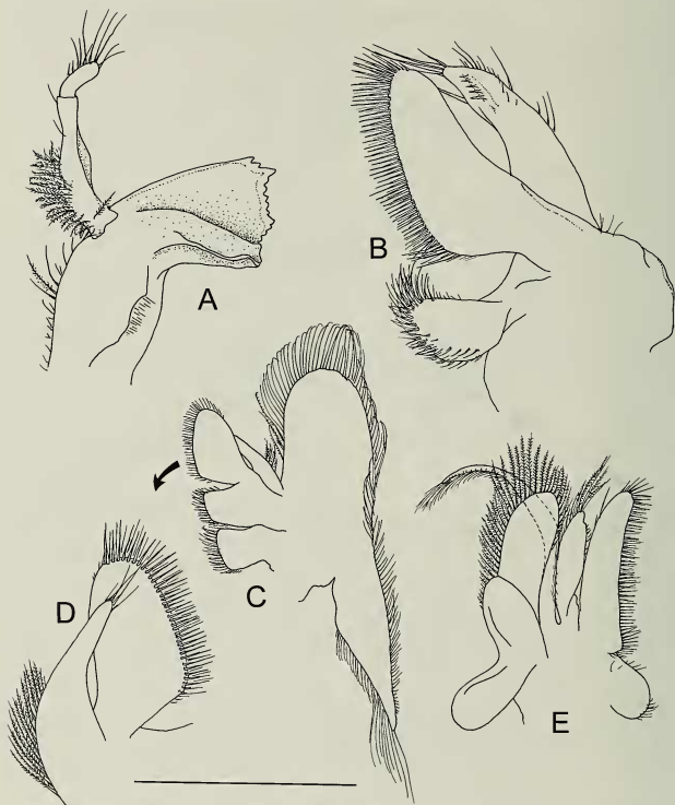
Fig. 3. Bathystylocladus echinus , new species, male paratype (LACM CR 1965-349.1). A. mandible; B. first maxilla; C. second maxilla; D. inner surface of second maxilla slightly enlarged and showing palp; E. first maxilliped. Scale bar = 5.0 mm A, B, D; 10.0 mm C, E.
